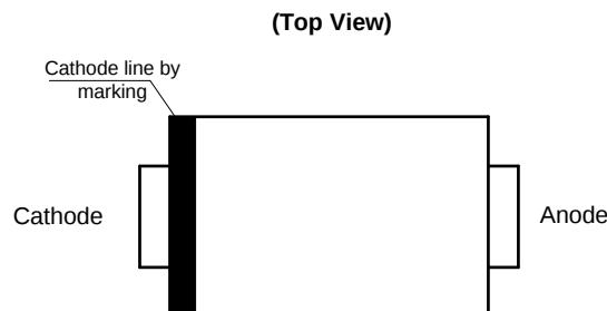
DO-214AC
